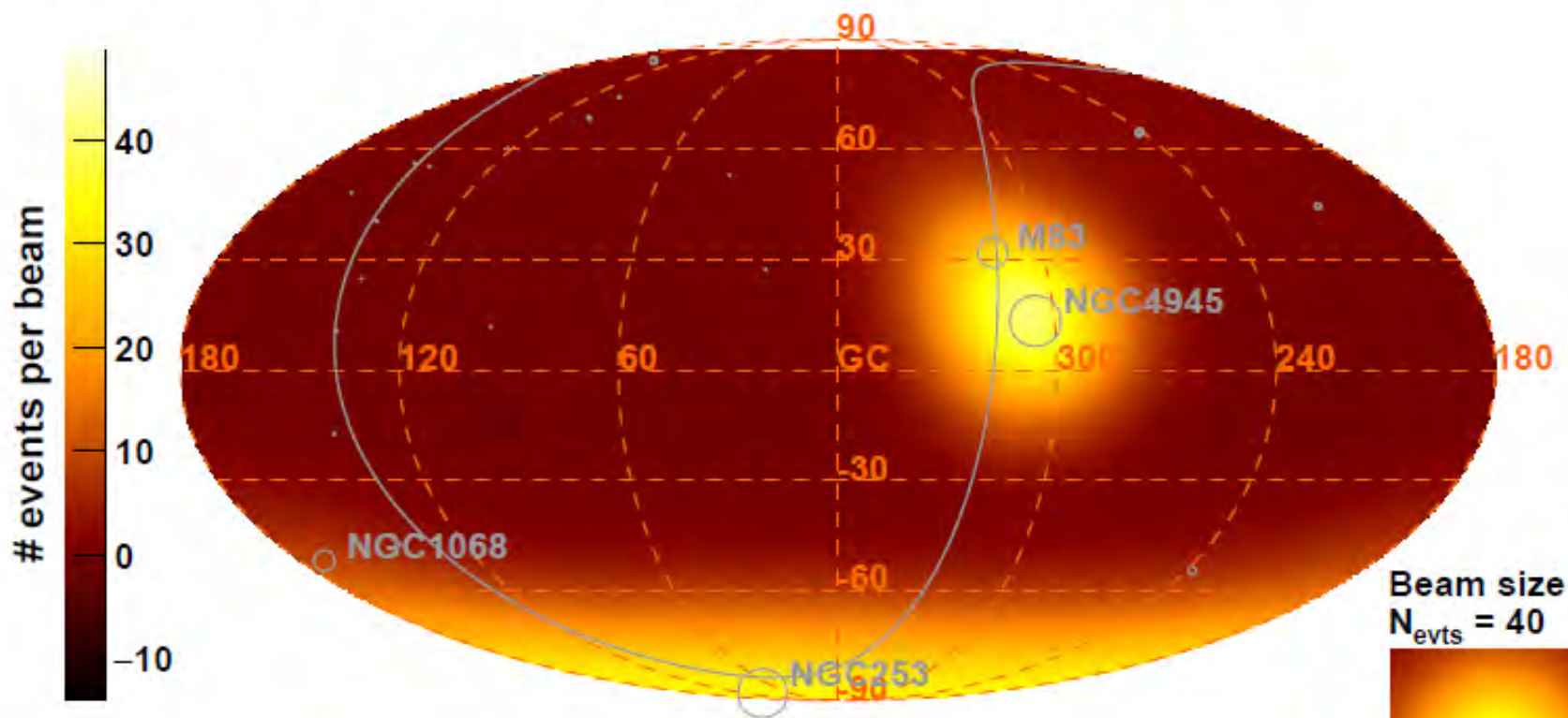
Model Excess Map - Starburst galaxies - E > 39 \text{ EeV}
